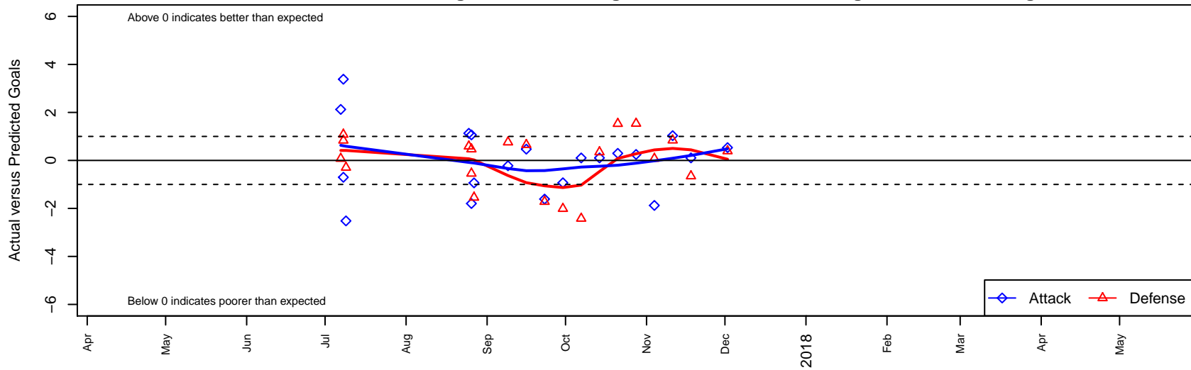
Highline SA B04 Dots are actual minus expected GF (blue circles) and GA (red triangles). Blue line is smoothed change in attack strength. Red is smoothed change in defense strength.
